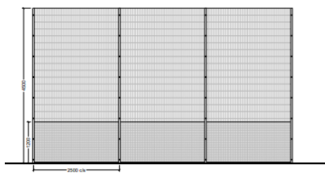
Detailed Elevation of 4.5m Surrounding Fence
